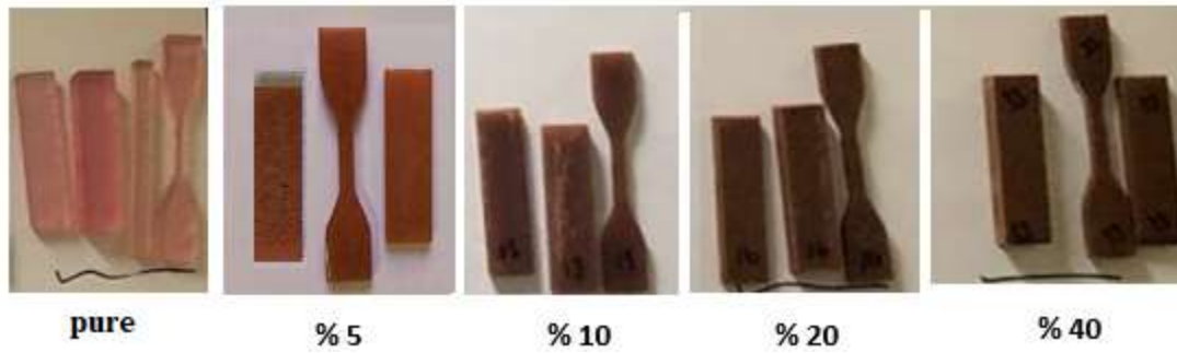
Fig. 3. Prepared specimens
