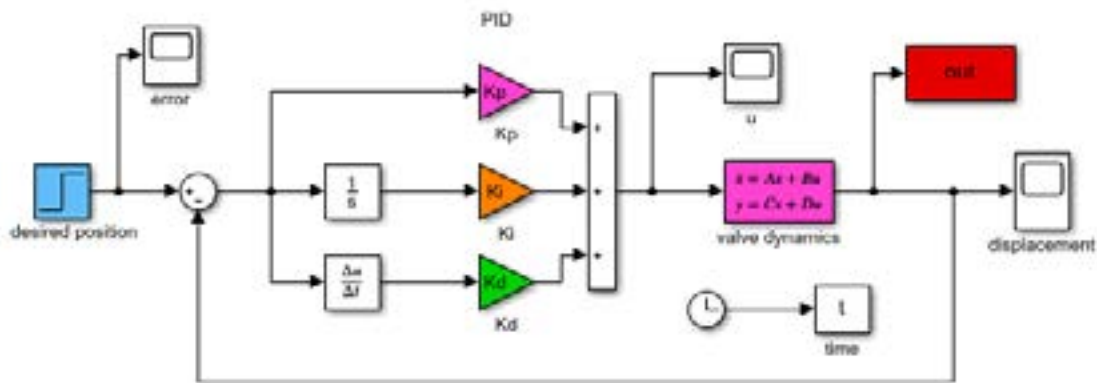
Figure 2. Control structure of the camless engine valve.
